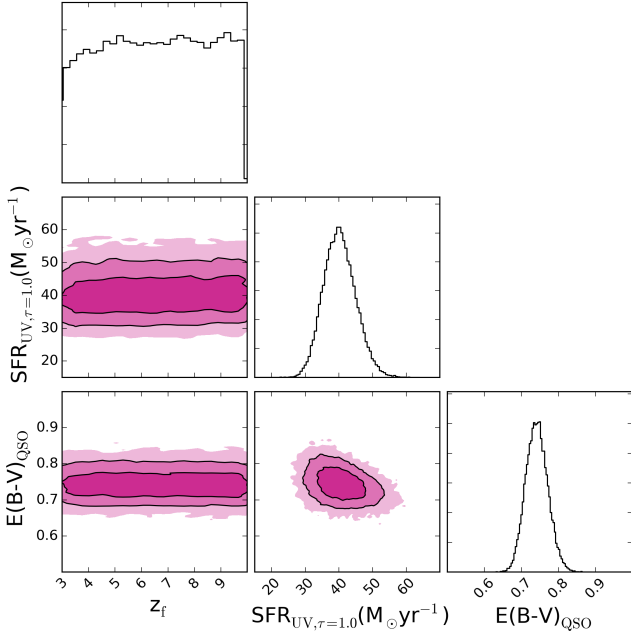
Figure 4. 1D and 2D posterior distributions from the MCMC fitting for VHSJ2235-5750 - a representative quasar from the sample. Shaded regions in the 2D distributions denote 1, 2 and 3\sigma parameter uncertainties in the fitting. The SFR and associated uncertainties (prior to dust corrections) are based on a galaxy template with \tau_V = 1.0 and have been converted from the normalisation of the galaxy template ( f_{\text{gal}} ) in the fitting. Histograms illustrate the relative 1D probability distributions of each parameter.
