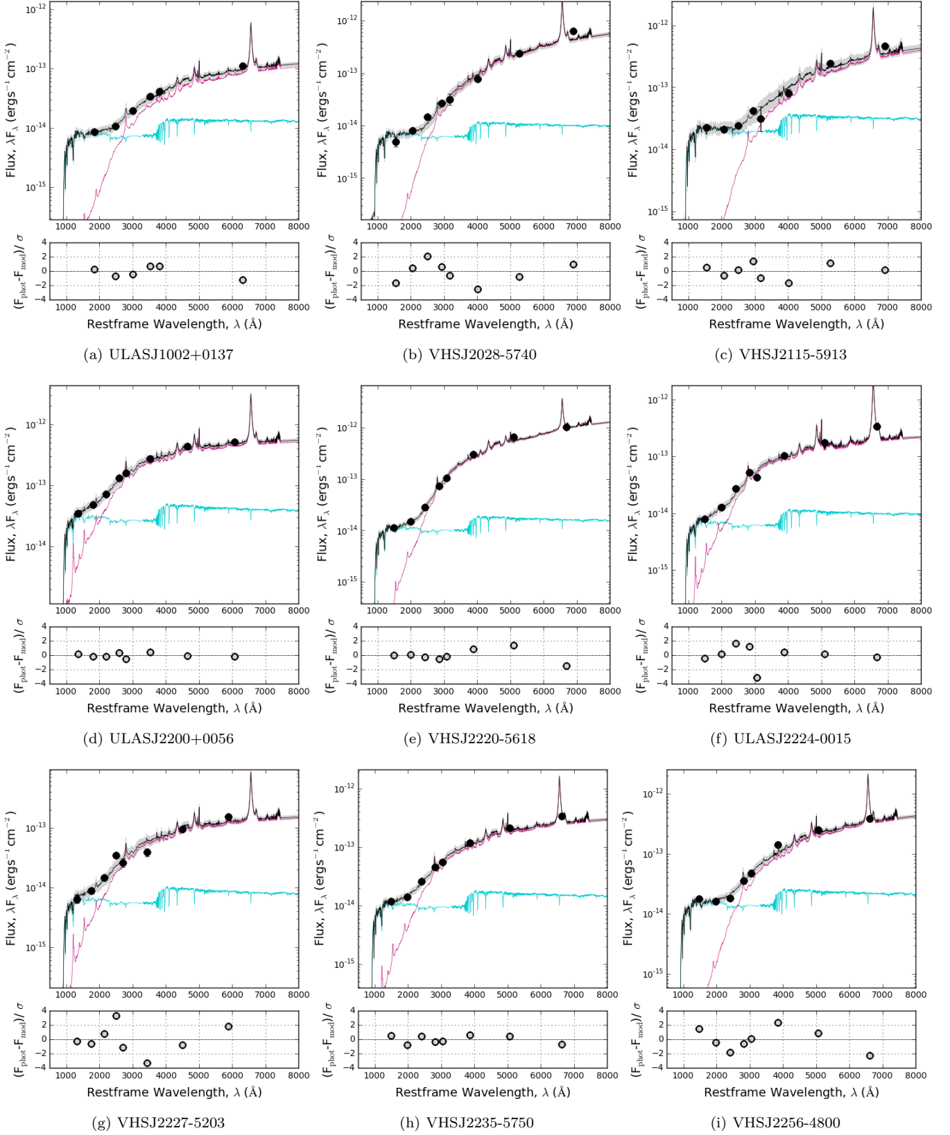
Figure 5. Upper panels: Best fit models (black) for the 13 reddened quasars with individual galaxy (blue) and quasar (pink) components overlaid. Black points show the grizY DES and JHK VHS/ULAS photometry. Grey shaded regions illustrate 1\sigma uncertainty about the best-fit model solution. Lower panels: Residuals for all photometric bands, scaled to the photometric errors (floored at 10 per cent).
