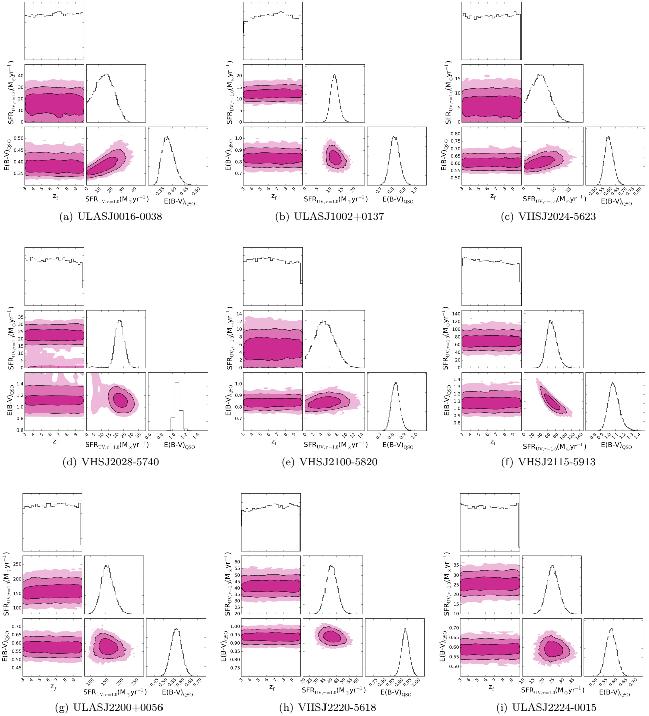
Figure A1. 1D and 2D posterior distributions from the MCMC fitting. Shaded regions in the 2D distributions denote 1,2 and 3\sigma parameter uncertainties in the fitting. \text{SFR}_{\text{UV},\tau_{\text{UV}}=1.0} and associated uncertainties (prior to dust corrections) are based on a galaxy template with \tau_{\text{UV}} = 1.0 and have been converted from the normalisation of the galaxy template ( f_{\text{gal}} ) in the fitting. Histograms illustrate the relative 1D probability distributions for each parameter.
