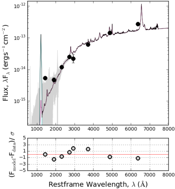
Figure 3. Best-fit model (black) for VHSJ2306-5447 with individual Lyman- \alpha (blue) and reddened quasar (pink) components overlaid.
