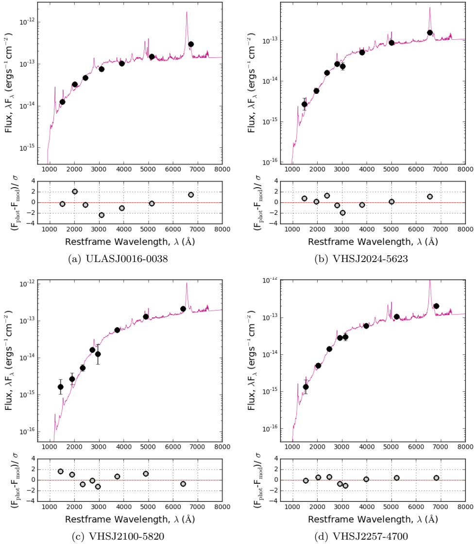
Figure 2. Upper panels: Best-fit quasar SEDs for ULASJ0016-0038 (a), VHSJ2024-5623 (b), VHSJ2100-5820 (c), VHSJ2257-4700 (d) for which \chi^2_{\text{red,QSO}} < 2.5 . Black points show the grizY DES and JHK VHS/ULAS photometry. Lower panels: The error-weighted residuals for each fit.
