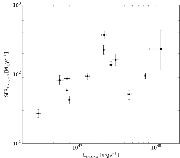
Figure 7. \text{SFR}_{\text{UV}} as a function of the dust-corrected L_{\text{bol,QSO}} . Error bars denote 1\sigma uncertainties on \text{SFR}_{\text{UV}} .
