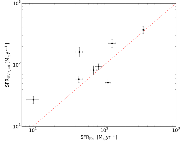
Figure 6. Comparison of \text{SFR}_{\text{UV}} to \text{SFR}_{\text{H}\alpha} ( Alaghband-Zadeh et al. 2016 ). Error bars show the 1\sigma uncertainties on the calculated SFRs in each case.
