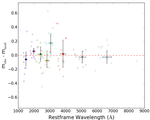
Figure 5. Magnitude differences between the fitted SED and the DES grizY photometry, assuming a galaxy template with \tau_V = 1.0 . Dark points denote the median average in each filter with error bars showing the median absolute deviation of the data points in each passband.
