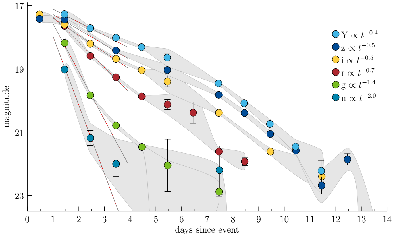
Figure 3. The observed light curve for the optical counterpart of GW170817 measured in 6 filters. The data points and 1\sigma error bars were measured using diffimg . The gray bands represent the 95% confidence interval about each measurement, or 2\sigma above sky if the measured flux is less than 2\sigma_{\text{sky}} . Data taken on days 5.5, 6.5 and 11.5 were obtained in poor weather conditions, hence the broader uncertainty bands. The photometry has been checked against a difference imaging reduction using Pan-STARRS PS1 templates (Cowperthwaite et al. 2017) and a galaxy fit & subtract PSF source magnitude reduction; these measurements are consistent with our results. The dashed lines show the initial decay of the source: m \propto t^{-\alpha} , where \alpha = (2.0, 1.4, 0.7, 0.5, 0.5, 0.4) in u,g,r,i,z,Y bands respectively. The decay in the first few days is consistent with a peak luminosity near t = 1 day. The table containing light curve information is available as a machine-readable file (Table 1).
