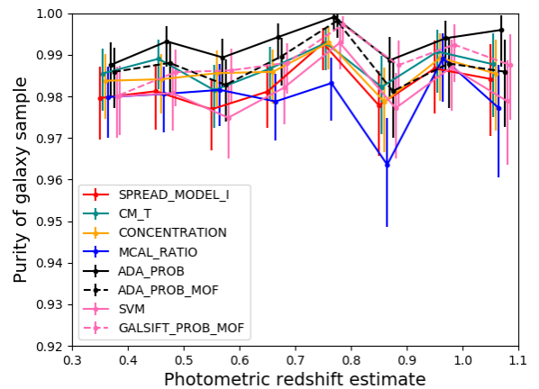
Figure 7. Purity of the galaxy sample as a function of photo- z for classifiers tested on Hubble-SC matches over the SN fields field, for a fixed 90% completeness. We use a random MonteCarlo sampling of the probability distribution function of redshift predicted by BPZ for that particular object as an estimate of its photo- z .
