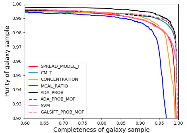
Figure 3. Precision-Recall (or completeness-purity) plot for classifiers tested on the SN fields over the Hubble-SC catalog, using galaxies as truth. Magnitude range is given by MAG\_AUTO\_I = (17,24) . The SPREAD_MODEL-based cut is similar to the MODEST_CLASS used in DES Y1 analyses.
