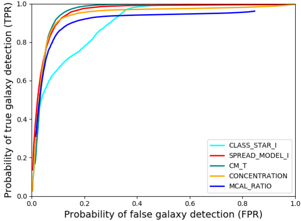
Figure 1. ROC plot for classifiers tested on the COSMOS field. Only non-ML codes are shown, as they are trained in this dataset. Magnitude range is given by MAG\_AUTO\_I = (17,24) . The SPREAD_MODEL-based cut is similar to MODEST_CLASS used in Y1 analyses. Galaxies are assumed to be the ‘truth’ for the purposes of the ROC definition.
