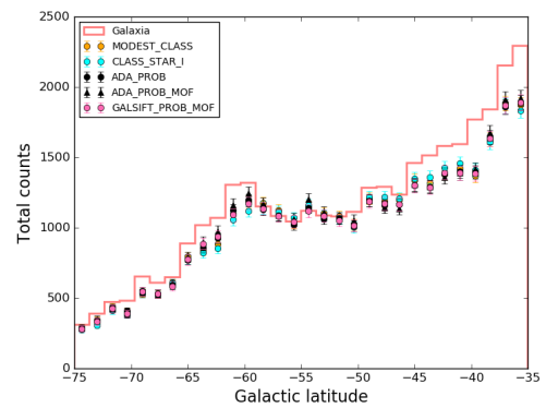
Figure 13. Counts for stars as classified by different algorithms compared to a Galaxia simulation (Sharma et al. 2011) for the application field of the DES-Y1 footprint for the magnitude range r = (19,21.5) .
