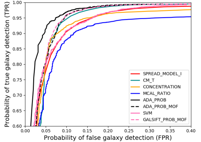
Figure 2. ROC plot for classifiers tested on the SN fields over the Hubble-SC catalog. Magnitude range is given by MAG\_AUTO\_I = (17,24) . The SPREAD_MODEL-based cut is similar to MODEST_CLASS used in Y1 analyses. Galaxies are assumed to be the ‘truth’ for the purposes of the ROC definition.
