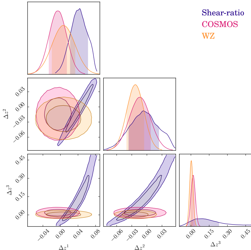
FIG. 12. Comparison of the constraints obtained on the source redshift distribution shifts using different methods: Shear-ratio test, photo- z studies in the COSMOS field (COSMOS, [32]) and cross-correlation redshifts (WZ, [33, 34]).
