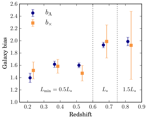
FIG. 14. Comparison of the galaxy bias results obtained from galaxy clustering measurements ( b_A , [35]) and from the galaxy-galaxy lensing measurements in this work ( b_\times ), by fixing all cosmological parameters to the 3x2 cosmology best-fit from [23]. The vertical dotted lines separate the three redMaGiC samples, which have different luminosity thresholds L_{\min} , defined in Sec. III A.
