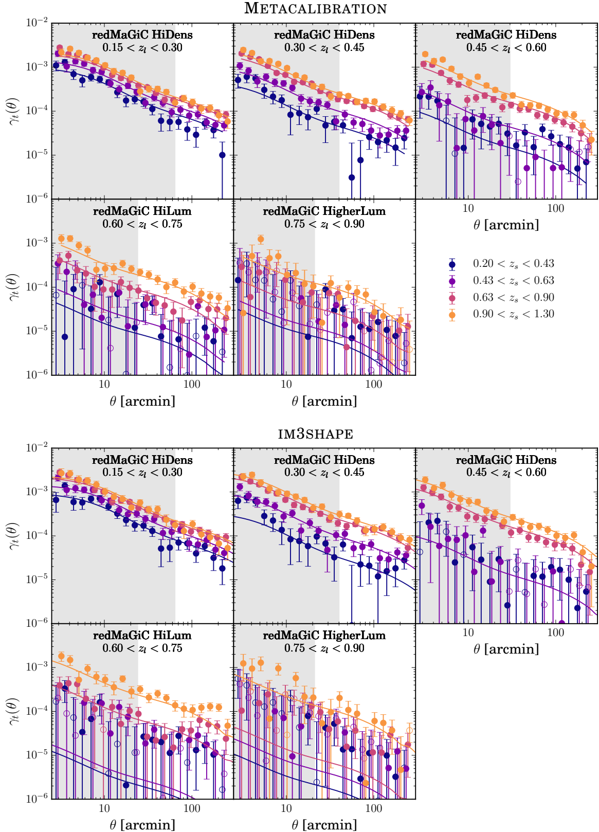
FIG. 2. Tangential shear measurements for METACALIBRATION and IM3SHAPE together with the best-fit theory lines from the DES Y1 multiprobe cosmological analysis [23]. Scales discarded for the cosmological analysis, smaller than 12 h^{-1}\text{Mpc} in comoving distance, but which are used for the shear-ratio test, are shown as shaded regions. Unfilled points correspond to negative values in the tangential shear measurement, which are mostly present in the lens-source combinations with low signal-to-noise due to the lenses being at higher redshift than the majority of sources. HiDens , HiLum and HigherLum correspond to the three redmagic samples (High Density, High Luminosity and Higher Luminosity) described in Sec. III A
