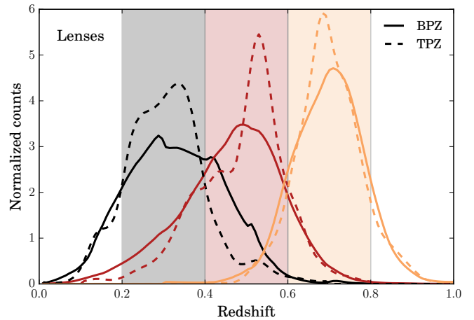
Figure 1. Normalized counts (or normalized N(z) 's) of the foreground redshift distribution of lens galaxies using two photo- z codes: BPZ and TPZ, also used in each case to define the galaxies that belong to each bin (as described in Table 1).
