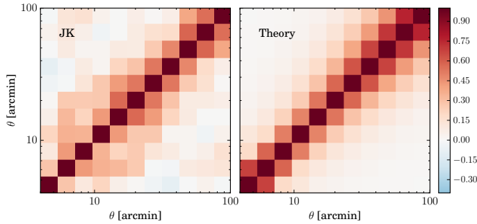
Figure 3. Correlation matrix (normalized covariance) for the mid- z lens bin defined with BPZ, with the mask applied. Left panel: Estimated with the jackknife method (Sec. 4.2.1). Right panel: Estimated with a theoretical modelling (Sec. 4.2.2).
