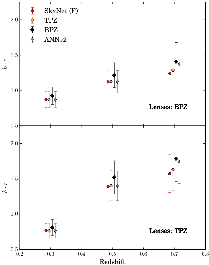
Figure 7. Galaxy bias results varying the photo- z code to estimate the redshift distribution of the source sample. For instance, for the red points, the N(z) of the sources is estimated with SkyNet (Fiducial). We observe good agreement among the different results. Top panel: Lens redshift bins are defined with BPZ and the lens N(z) is estimated using BPZ as well. Bottom panel: The same with TPZ. NGMIX is the source catalog used for these results. The points have been offset horizontally for clarity purposes.
