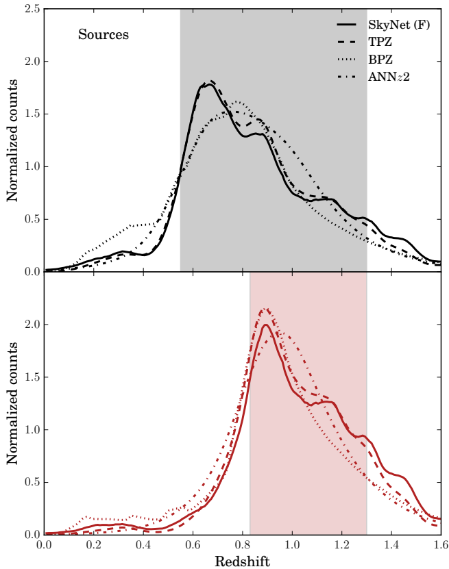
Figure 2. Normalized counts (or normalized N(z) 's) of the background redshift distribution of source galaxies from NGMIX using the following four photo- z codes: SkyNet, TPZ, BPZ and ANNz2, for both source redshift bins: 0.55 < z_{\text{SkyNet}} < 1.3 ( upper panel ) and 0.83 < z_{\text{SkyNet}} < 1.3 ( bottom panel ). We choose SkyNet to be the fiducial photo- z code to estimate the N(z) of the source galaxies.
