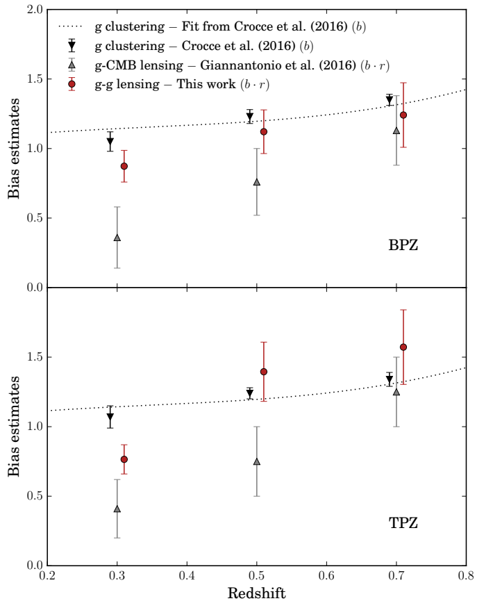
Figure 8. Fiducial galaxy bias results from this work using galaxy-galaxy lensing (g-g lensing, red points) as a function of redshift compared with previous measurements on the same Benchmark sample using galaxy clustering (g clustering, black down triangles) from Cr16 and the real space analysis results from CMB lensing (g-CMB lensing, gray upper triangles) from G16. Top panel: Lens redshift bins are defined with BPZ and the lens N(z) is estimated using BPZ as well. Bottom panel: Lens redshift bins are defined with TPZ and the lens N(z) is estimated using TPZ as well. The points have been offset horizontally for clarity purposes.
