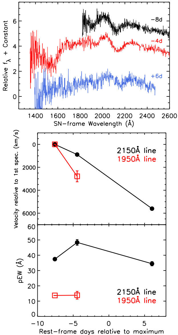
Figure 4. Top: Spectra of DES15E2mlf focusing on the two strong absorption features at \sim 1950 Å and 2150 Å. Middle: Velocity of the 2150 Å (black circles) and 1950 Å (red open squares) absorption lines relative to the velocity in the first epoch as a function of phase. Bottom: Pseudo-equivalent width (pEW) for the two features as a function of phase.
