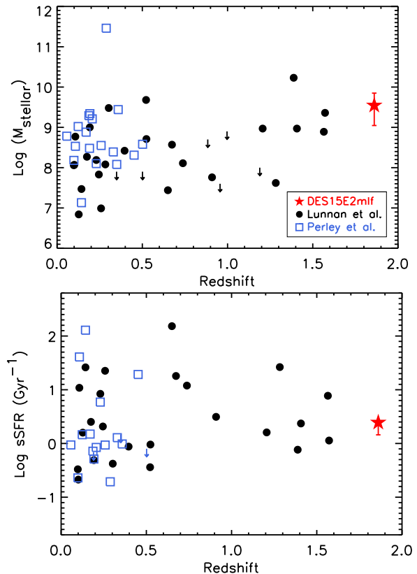
Figure 7. SLSN-I host-galaxy M_{\text{stellar}} as a function of redshift (top panel) and sSFR as a function of redshift (bottom panel). Black points and blue squares represent the Lunnan et al. (2014) and Perley et al. (2016) sample, respectively, while the red star represents the host galaxy of DES15E2mlf.
