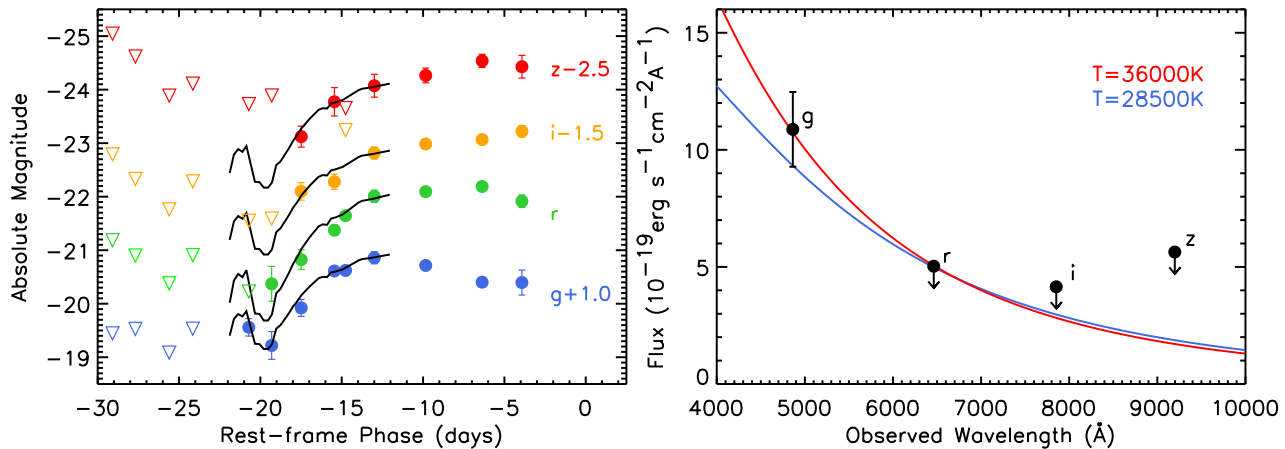
Figure 8. Left: A closer look at DES15E2mlf pre-maximum light curves. The upper limits are shown in downward triangles. We overplot the scaled LSQ14bdq rest-frame g -band light curve (Nicholl et al. 2015) in black. Right: The DES15E2mlf g -band flux and upper limits for riz bands at -21 days. The blackbody curves with T = 28,500 \text{ K} (blue) and 36,000 \text{ K} (red) are overplotted.
