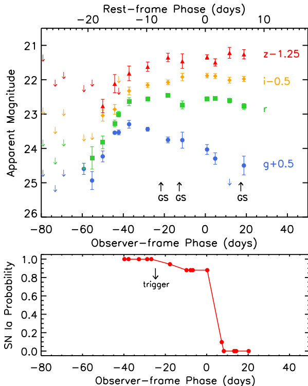
Figure 1. Top: DECam griz light curves of DES15E2mlf. The phase of observation is relative to the peak of the i -band light curve on MJD = 57384.26. Upper limits are represented by the downward arrows. The upward arrows in black mark the epochs of Gemini-South spectra. Bottom: pSNID (Sako et al. 2008, 2011) probability of DES15E2mlf being a SN Ia as a function of phase. The arrow indicates the epoch when we triggered the first spectrum.
