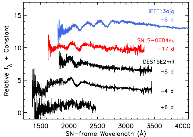
Figure 2. Gemini-South spectra of DES15E2mlf (black) at -8 , -4 and +6 days relative to peak i -band brightness. We also display the spectra of iPTF13ajg (blue) and SNLS-06D4eu (red), SLSNe-I at z = 0.740 and 1.588 , respectively.
