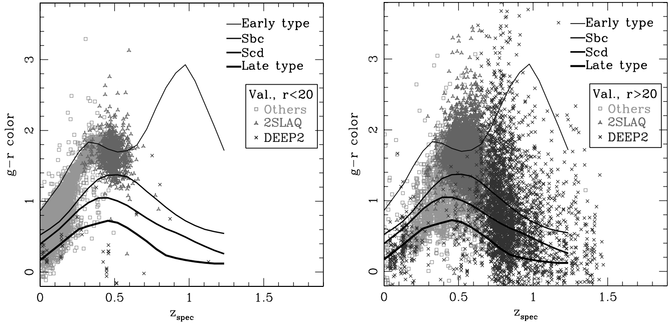
FIG. 7.—The g-r color vs. spectroscopic redshift for galaxies in the validation set. Left: Galaxies with r < 20 . Right: Galaxies with r > 20 . The solid curves show expected color-redshift relations of galaxies with different SED types, calculated using the Coleman et al. (1980) spectral templates. The different shades of gray indicate galaxies from the different spectroscopic surveys that contributed to the validation set. The 2SLAQ objects, denoted by triangles, were selected to be mostly early-type galaxies. They are responsible for the minimum in \sigma vs. z_{\text{spec}} for the r > 20 subsample in Fig. 6. [See the electronic edition of the Journal for a color version of this figure.]
