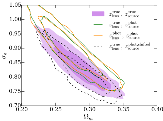
Figure 4. The impact of using photometric redshift estimates. For all contours, the datavector is the mean of all BCC realizations. Purple filled contours use the true redshift distributions for both lens and source galaxies. Note in this case galaxies are binned according to their photo- z , but the n(z) for each redshift bin is estimated using true redshifts. The green unfilled contours use source redshift distributions estimated using BPZ photo- z s, while the orange unfilled contours additionally use the photometric redshift estimates from the the REDMAGIC algorithm, z_{\text{RM}} for the lenses. The black dashed contours use BPZ to estimate the source n(z) s, shifted in redshift to have the correct mean (see Section 5.4 for details).
