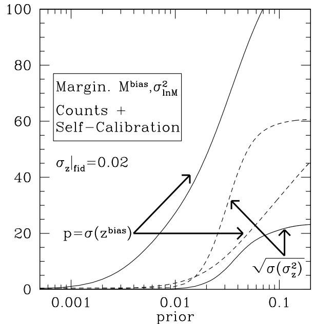
FIG. 7: Dark energy parameters degradation for a fiducial photo- z scatter of \sigma_z|_{\text{fid}} = 0.02 constant in redshift as opposed to the fiducial model of Eq. (28).
