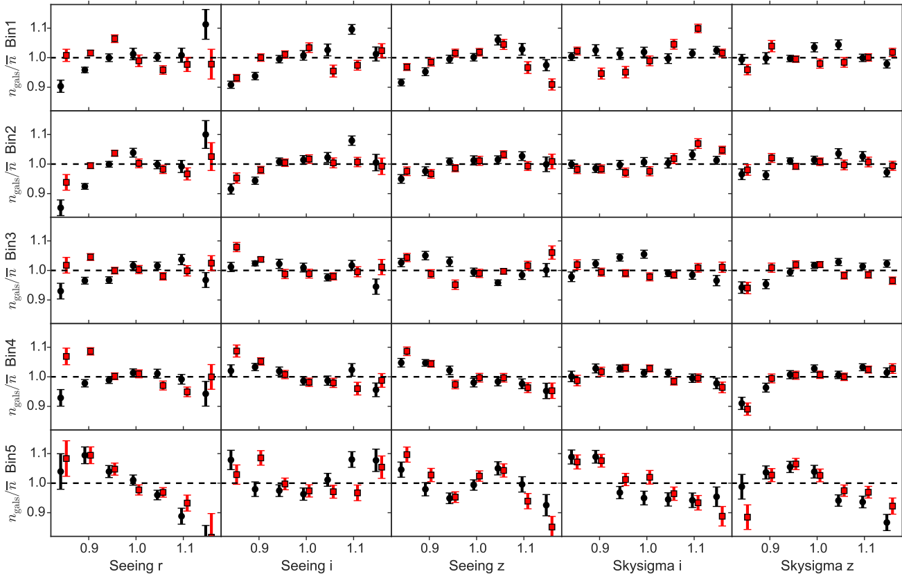
Figure 11. Changes in the galaxy number densities ( n_{\text{gals}} ) relative to the mean ( \bar{n} ) in each redshift bin, as a function of some observational properties, also normalised to their mean values. Both the SV data (black circles) and BCC-UFig (red squares) exhibit similar fluctuations, which are small but significant compared to the sample variance, calculated using jack-knife re-sampling in 50 sky regions.
