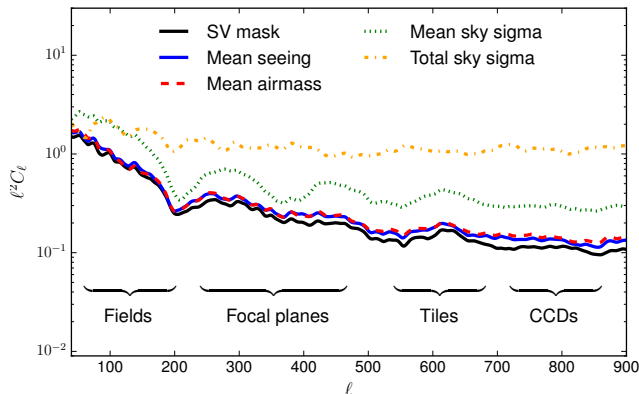
Figure 5. Full-sky angular power spectra of some of the i band observational systematics shown in Figure 4. Prior to power spectrum estimation, the maps were divided by their average values in order to obtain dimensionless C_\ell 's. The power spectrum of the DES-SV coverage mask (presented in Rykoff et al. 2015; Crocce et al. 2015) is also shown in black. Any excess of power relative to the mask implies structure and features in the maps, which can yield non-trivial contamination and systematics in the galaxy catalogues. We also indicate the characteristic scales affected by the geometry of the SV survey and DECam instrument.
