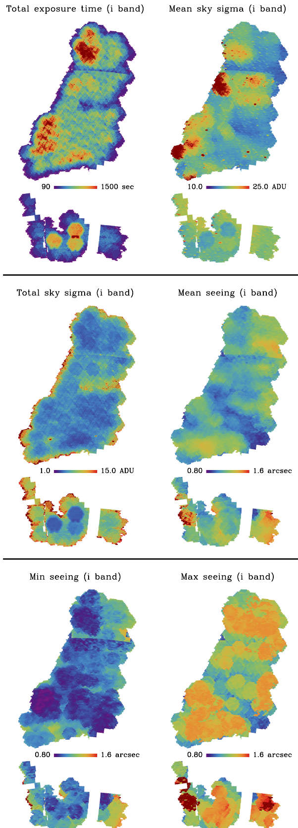
Figure 4. Maps of some of the main observational quantities (potential sources of systematics) in the SPT-E and W fields (top and bottom of each sub-panel). The HEALPix maps are produced at N_{\text{side}} = 4096 , where each pixel is the mean value of the observed N_{\text{side}} = 16384 sub-pixels, in order to obtain more accurate values near the edges of the survey.
