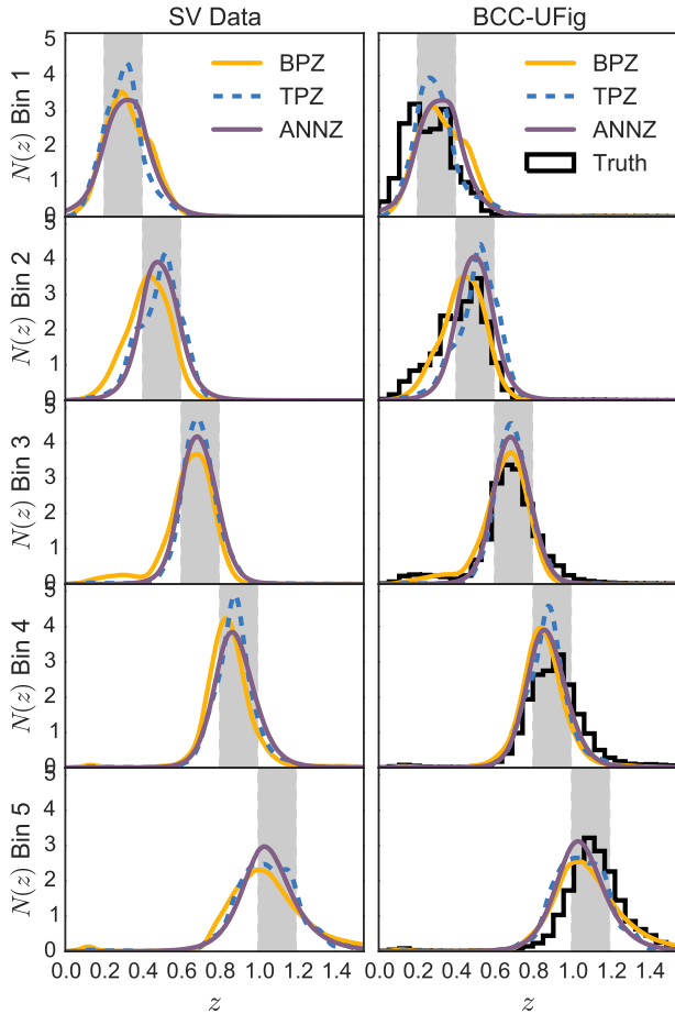
Figure 8. Redshift distributions of the SV data (left) and BCC-UFig (right) catalogues obtained using the photometric redshift estimation methods trained on a spectroscopic sample of galaxies (see text for details). They are normalised such that \int N(z)dz = 1 . By comparison, the variance obtained by randomly splitting the redshift samples is of the order of 0.01 in all redshift bins.
