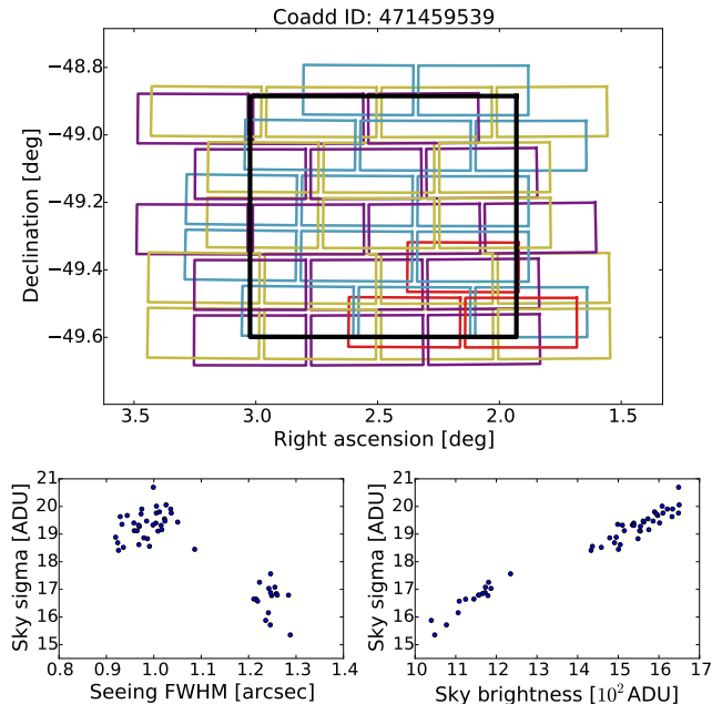
Figure 1. Upper panel: geometrical projection of the single-exposure images coadded in an arbitrary tile of the DES Science Verification data (black contour). The colours correspond to different single-epoch pointings, with the relevant CCDs shown as individual rectangles. Lower panels: properties of the same set of CCDs, exhibiting significant variations and correlations. The nontrivial, spatially-varying geometrical overlap and image properties will result in spatially-varying systematics when analysing the galaxy catalogues.
