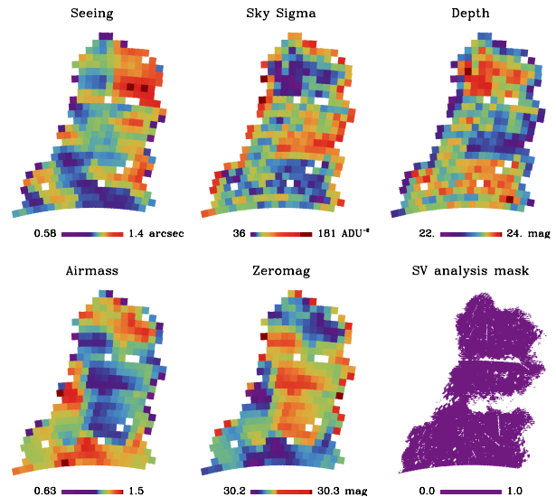
Figure 7. Maps of the i band SV observing conditions incorporated in the BCC-UFig simulation, obtained by smoothing the maps of Figure 4 in tiles. The analysis mask shows the region considered when measuring the redshift distributions and galaxy number densities presented below.
