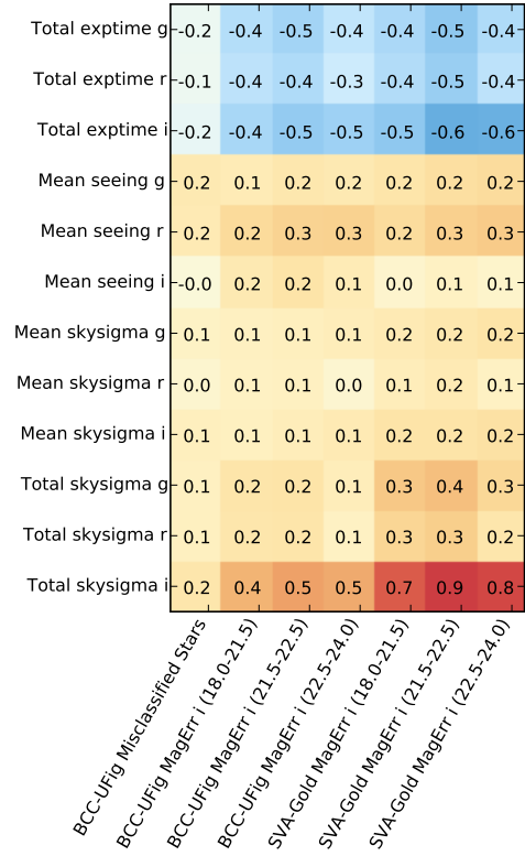
Figure 12. Pearson correlation coefficients between observing conditions, stars misclassified as galaxies in the BCC-UFig reduced data, and mean i band magnitude errors ( mag_err_auto.i ) in both the BCC-UFig and SVA1-Gold galaxy catalogues (in magnitude bins, using mag_auto.i ). This shows that the maps of the observing conditions are significantly correlated with the stellar contamination and depth fluctuations in the SV data and simulations, therefore capturing the main sources of spatial systematics present in the galaxy samples.
