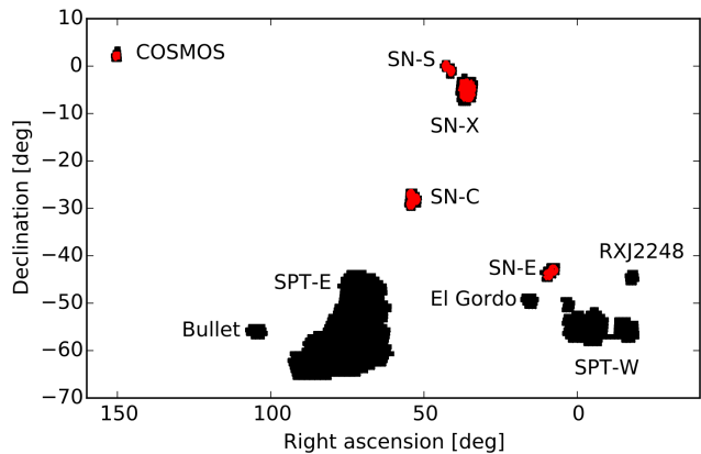
Figure 3. The DES SV footprint, partitioned into several discontinuous regions, the largest being the SPT-E and W fields ( \approx 200 and 50 \text{ deg}^2 , respectively). The small red regions contain objects where spectroscopic redshifts are available, used to train the photometric redshift estimation codes, as discussed in Section 3.
