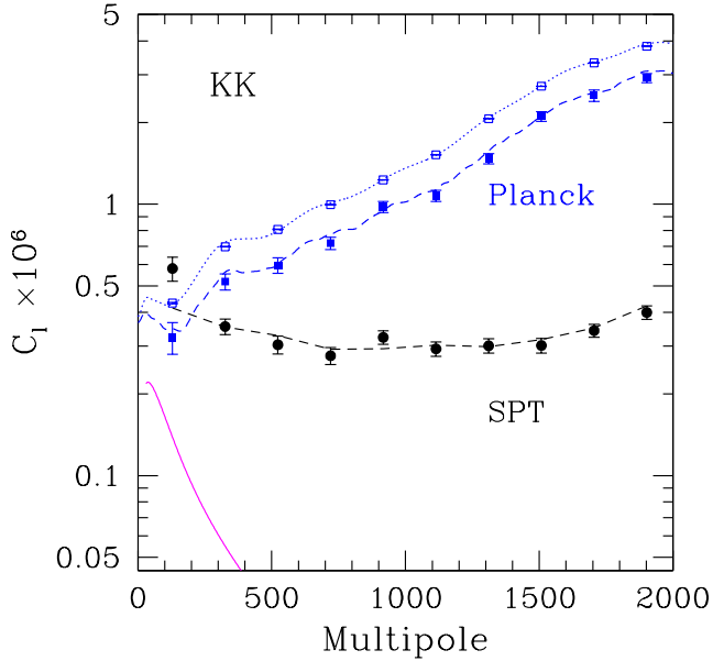
Figure 9. Auto-spectra measured from the CMB lensing convergence maps (points with error bars) from Planck (blue squares) and SPT (black circles), compared with the fiducial cosmological signal (magenta solid line). The dashed lines describe the average of 100 mock realisations that fully characterise the Planck and SPT maps respectively. For the Planck case we show two sets of data: measured over the full Planck lensing mask (dotted line and empty points), and over the intersection of the lensing mask with the DES-SV SPT-E mask (dashed line, full points). We can see that the convenient position of the DES-SV SPT-E area next to the South Ecliptic Pole results in a 25% noise reduction. No smoothing is applied to the maps for this figure.
