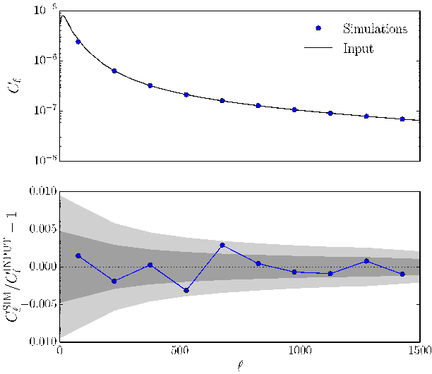
Figure D1. The optimal quadratic estimator is unbiased. We compare the power spectra estimates, averaged over all 1000 simulations, to the input power spectrum ( top panel ). We also plot the residuals after dividing by the fiducial model ( bottom panel ) together with the 1 and 2- \sigma error on the mean ( grey regions ), i.e., the error bars of an individual simulation divided by \sqrt{1000} . We find no evidence for a detectable bias, even in the highest multipole bins close to the resolution limit of a HEALPIX map at N_{\text{side}} = 512 .
