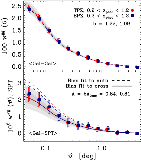
Figure 19. Measured DES auto- ( top ) and DES-SPT lensing cross-correlation ( bottom ) functions for two different choices of photometric redshift estimators: our baseline TPZ choice is shown in red, while the alternative BPZ catalogue is in navy blue. The theory lines are produced accordingly to each catalogue’s redshift distribution. The recovered best-fit biases and cross-correlation amplitudes are shown in the caption for both photo- z methods.
