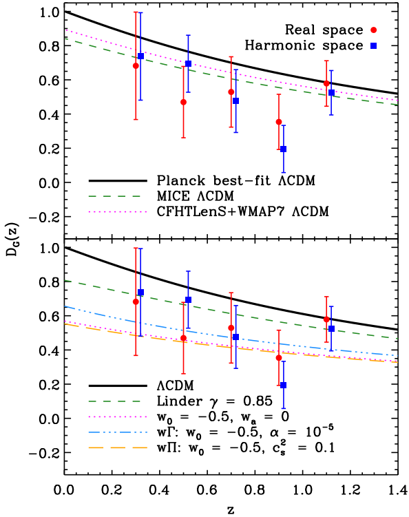
Figure 22. The red circles and blue squares show our growth function measurements with the D_G estimator, compared with the fiducial Planck best fit \Lambda CDM prediction (thick black line), different choices of the \Lambda CDM parameters ( top panel ), and a selection of dark energy and modified gravity models ( bottom panel ). Top panel : The green dashed line shows the prediction for the MICE cosmology, while the orange dot-dashed line refers to the best-fit \Lambda CDM model to the CFHTLenS + WMAP7 data by Heymans et al. (2013) . Bottom panel : The coloured lines display in the order: a Linder \gamma model ( Linder & Cahn 2007 ), a dark energy model parameterised by w_0, w_a ( Chevallier & Polarski 2001 ), and two models of modified gravity at the perturbative level: entropy perturbation ( wI ) and anisotropic stress models ( wII ), as described by Battye & Pearson (2013) .
