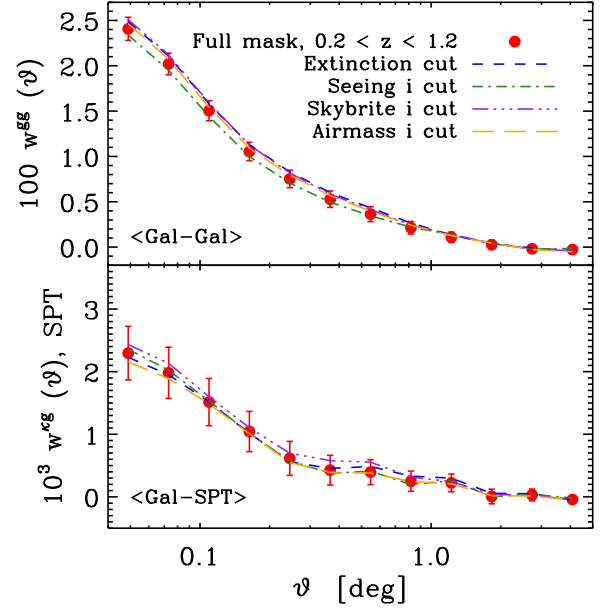
Figure 16. Measured DES auto- (top) and cross- (bottom) correlation functions with SPT lensing obtained from the full mask (red dots) and applying cuts in the main contaminants we consider (coloured lines). For each potential systematic, we remove 20% of the area, corresponding to the most affected regions. The results are stable: the correlation functions do not deviate significantly compared with the statistical error bars.
