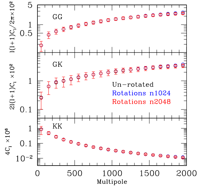
Figure A1. Comparison between the rotated and un-rotated (all-sky) power spectra (from top to bottom: galaxy-galaxy, galaxy-CMB lensing, and lensing-lensing). Rotated mocks (in blue and red for N_{\text{side}} = 1024, 2048 respectively) yield unbiased results with respect to the un-rotated maps (black). The Gaussian smoothing was not applied for this particular test.
