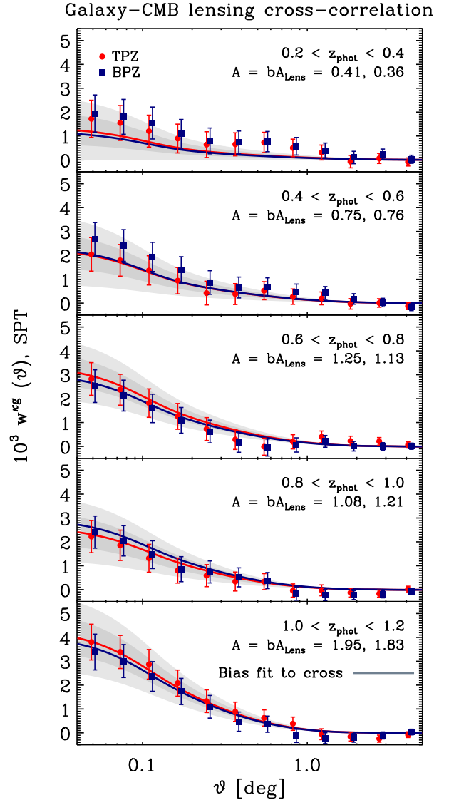
Figure 20. Redshift tomography using two different photo- z methods: TPZ ( red ) and BPZ ( navy ). The theoretical curves and best-fit amplitudes for the cross-correlations are also shown for each method. The recovered results agree. See Crocce et al. (2015) for similar tests on the galaxy auto-correlations. In the first photo- z bin at 0.2 < z_{\text{phot}} < 0.4 the best fit curves do not trace the data closely, given the mismatch between the measurements and the template shape, and the high covariance between the points.
