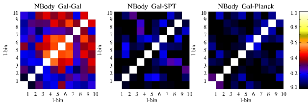
Figure 8. Correlation matrices from N -body realisations in harmonic space: we show correlations among C_\ell band-powers for the galaxy auto-, galaxy-SPT lensing and galaxy- Planck cross-correlations, from left to right, respectively. We use ten linear multipole band-powers with \Delta\ell = 197 .
