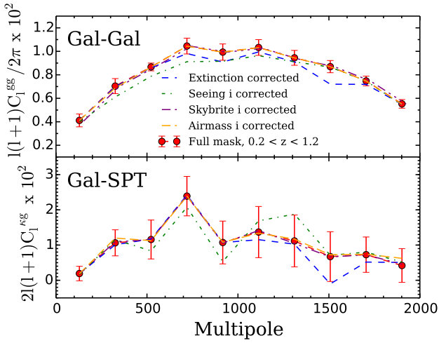
Figure 17. The galaxy-galaxy ( top ) and galaxy-SPT lensing ( bottom ) power spectra, including systematic corrections. Corrections are overall small, and especially so for the cross-spectrum, with all data points within 1\sigma in this case. The best-fit bias and level of detection are negligibly changed when including these corrections.
