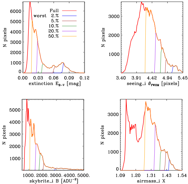
Figure 15. Pixel distributions of the potential DES systematics we consider. The histograms show the number of pixels where each systematic assumes the value shown in the abscissa. In addition, five possible cuts of the worst affected areas are shown, ranging from 2 to 50%.
