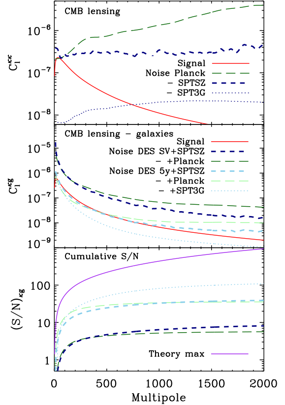
Figure 1. Signal-to-noise forecasts for the DES-CMB lensing correlations, for a range of different CMB and DES data sets. Top panel: The theoretical CMB lensing auto-spectrum compared with the noise of Planck 2015 and SPT-SZ as well as the projected noise of the upcoming SPT-3G survey. Central panel: The theoretical CMB lensing-galaxy cross-spectrum compared with the analytical errors estimated for the Planck and SPT cases, considering DES SV (top, darker colours) and 5-year data (bottom, lighter colours). The errors are large as they are shown per individual multipole \ell , and are correspondingly reduced once binned. Bottom panel: The cumulative signal-to-noise ratio of the CMB lensing-galaxy cross-correlations for the same cases, compared with the theoretical maximum fixed by cosmic variance. Note that a 5-10 \sigma detection is expected for SV data with the information coming from \ell < 2000 . For the full DES 5-year data, the measurement with Planck is expected to yield a similar significance to SPT-SZ, given the larger overlapping area. SPT-3G will achieve the most accurate measurement.
