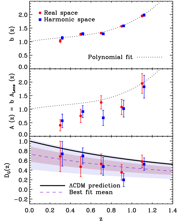
Figure 21. Reconstructed measurements of the redshift evolution of linear bias b(z) from galaxy auto-correlations, as also presented by Crocce et al. (2015) (top panel), galaxy-CMB lensing cross-correlation amplitudes A(z) from the cross-correlations (central panel) and linear growth function from the D_G(z) estimator (bottom panel) from the combined tomography of galaxy clustering and galaxy-CMB lensing correlations. The red (round) points are derived from the correlation functions, while the blue (square) points are from the angular power spectra. The purple dashed line shows the mean best fit amplitude to D_G with 1 and 2\sigma uncertainty bands. We also show for comparison the best-fit bias model of Eq. (34) in the top and central panels (dotted lines), and the theoretical growth function for the Planck fiducial cosmology in the bottom panel (thick solid line). The low values of A we observe translate into a preference for a lower D_G in most redshift bins.
