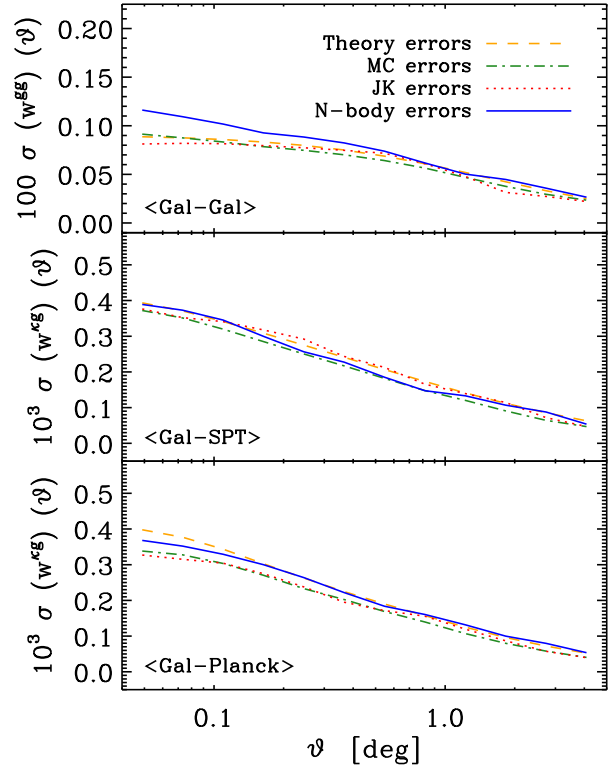
Figure C1. Comparison of the real-space diagonal error bars for our four estimators of the covariance matrix: theoretical (orange dashed), MC (green dot-dashed), JK (red dotted) and from N -body simulations (blue solid). The three panels refer from top to bottom to galaxy auto-correlation, and the cross-correlations with SPT and Planck . The different methods agree for the cross-correlations, while the N -body covariance yields marginally larger error bars for the auto-correlation as expected due to the effect of non-Gaussianities. We use the N -body errors for our main results.
