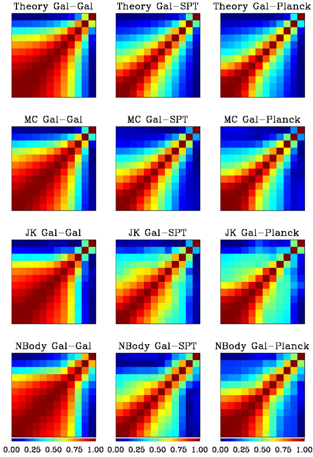
Figure C2. Comparison of four correlation matrix estimators in real space, for the three correlations we consider. The first row refers to the theoretical covariance, the second row is obtained from 1000 MC realisations, the third row is the JK method (100 regions), and the final row shows the 100 N -body realisations. The three columns refer to galaxy-galaxy, galaxy-SPT and galaxy-Planck lensing convergence correlations respectively. The angular range is from 2.4 arcmin to 5 deg as in Fig. 5. The different methods produce consistent covariances; by comparing the different correlation matrices, we see that the galaxy-CMB lensing correlation matrices are more diagonal than the galaxy-galaxy case, which is related to the auto-correlation theory being more non-linear, and thus more non-Gaussian and covariant, at these scales. Furthermore, all matrices become more covariant in the first few angular bins due to the introduction of the Gaussian smoothing to the maps, which effectively blurs information on scales \vartheta < \vartheta_{\text{FWHM}} = 5.4' (DES-SPT) and \vartheta < \vartheta_{\text{FWHM}} = 10.8' (DES-Planck).
