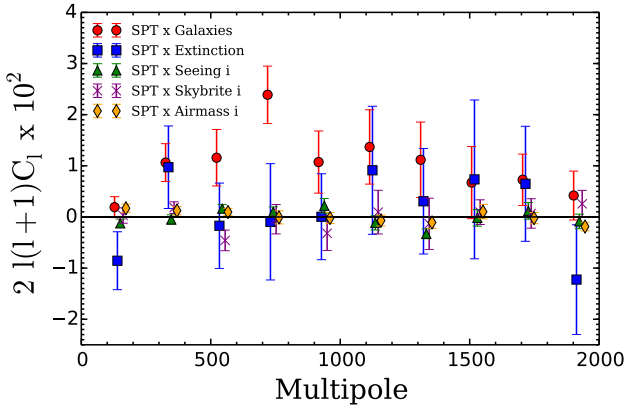
Figure 18. Correlations between the SPT convergence map and the potential systematic maps. Data points are offset on the x -axis for clarity. The galaxy-lensing correlation ( red circles ) is detected at 6\sigma , while the majority of the SPT cross systematic maps data points are consistent with zero. Correlating the SPT maps with DES potential systematic maps is expected to produce a null result, which we recover.
