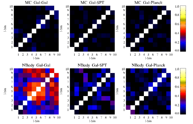
Figure C3. Comparison of two different correlation matrix estimators in harmonic space: the first row shows the results from MC realisations, while the second row refers to 100 N -body realisations. We show correlations among C_\ell band-powers for the galaxy auto-, galaxy-SPT lensing and galaxy-Planck cross-correlations, from left to right, respectively. We use ten linear multipole band-powers with \Delta\ell = 197 .
