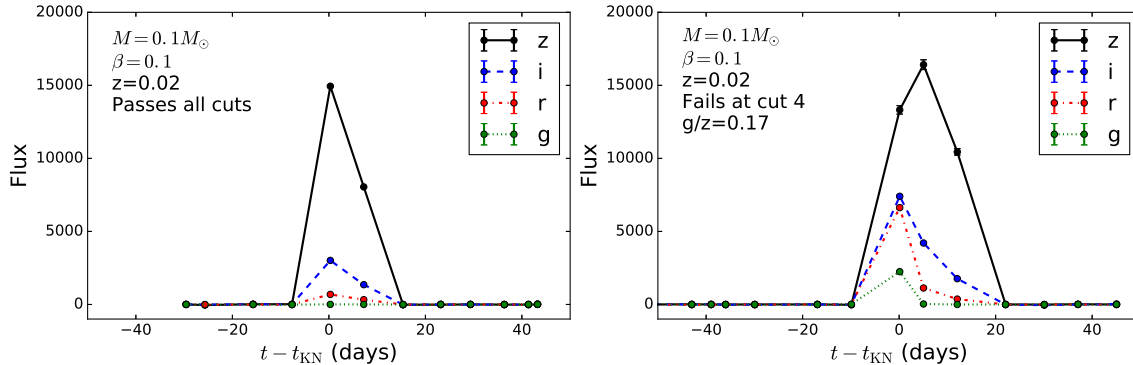
Figure 6. Example griz \beta = 0.1 , M = 0.1M_{\odot} light curves at magnitude 18 that pass the cuts (left) and fail the cuts at cut 4 (right). The points show the observed fluxes and lines are drawn between them to guide the eye. Fluxes are defined such that magnitudes are given by 27.5 - 2.5 \log_{10}(\text{Flux}) ; e.g., \text{mag}=22.5 for \text{Flux}=100 .
