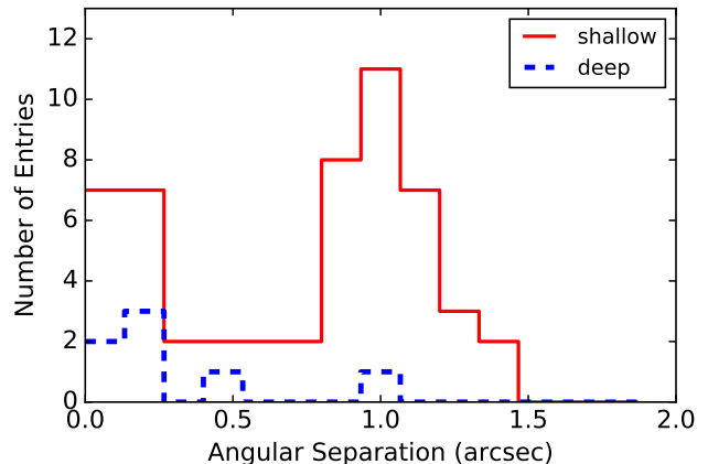
Figure 3. Distributions of the angular separation between KN trigger i and z observations \delta_{iz} for the DES-SN data. The first ten cuts are applied. A few objects with outlying \delta_{iz} are not shown on the plot.
