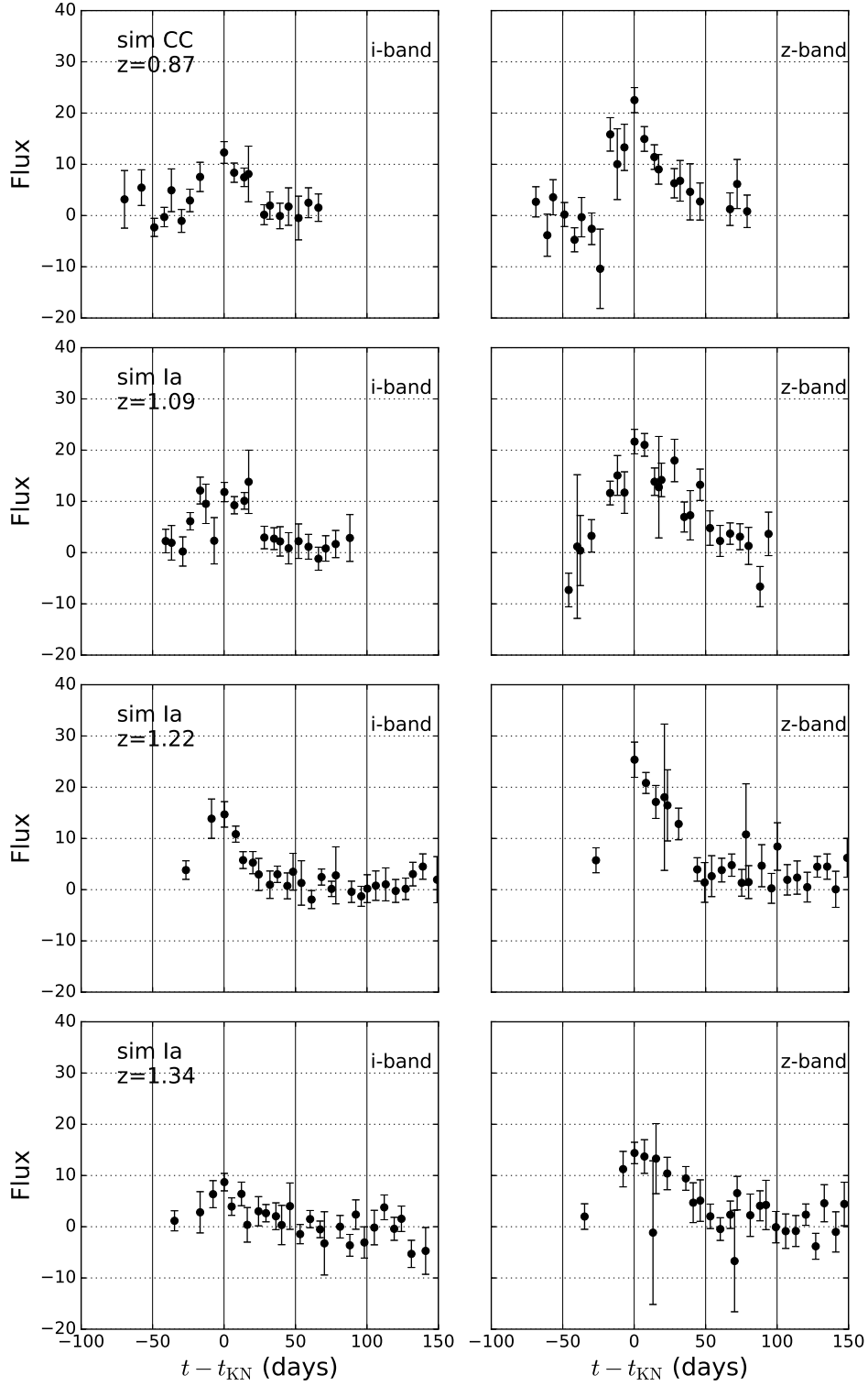
Figure 11. Example i and z -band light curves for simulated CC and Ia which passed all cuts. Fluxes are defined such that magnitudes are given by 27.5 - 2.5 \log_{10}(\text{Flux}) ; e.g., \text{mag}=25 for \text{Flux}=10 .
