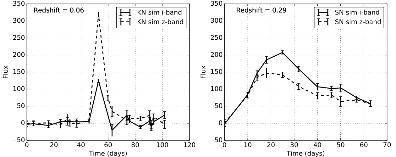
Figure 2. Observed KN and SN light curves in the i and z filters, as simulated with SNANA . The KN is based on the BK13 model with \beta = 0.3 , M = 0.1M_{\odot} and redshift z = 0.06 . The SNIa is simulated with SALT-II color c = 0.03 , stretch parameter x_1 = -0.75 , and redshift z = 0.29 . Magnitudes are given by 27.5 - 2.5 \log_{10}(\text{Flux}) ; e.g., the shallow-field detection limit of \text{mag}=23.5 corresponds to \text{Flux}=40 . The error bars show the simulated flux and uncertainties for each observation; the lines connect these simulated points to guide the eye.
