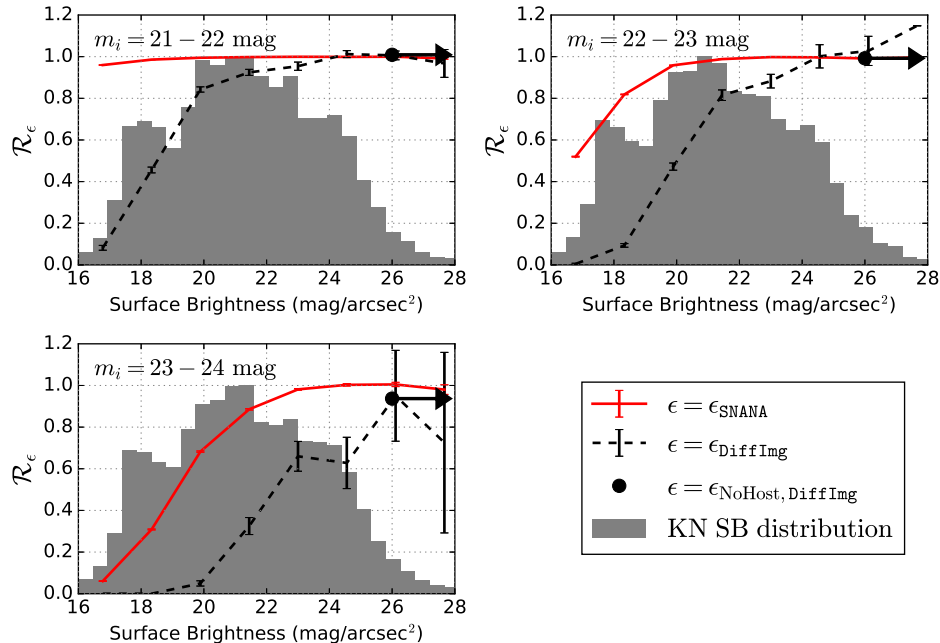
Figure 7. \mathcal{R}_e in the DES-SN shallow fields vs. m_{\text{SB}} for KN i -band magnitudes (a) m_i = 21-22 , (b) 22-23 , and (c) 23-24 . The solid red line is based on the SNANA simulation, and the dashed black line is from fake point sources processed by DiffImg. The gray regions show the i -band surface brightness distribution in the shallow-field, calculated in SNANA from the DES+2MASS catalogue Sersic profiles. The black dot and arrow shows \mathcal{R}_e for DiffImg fakes with m_{\text{SB}} > 26 , i.e. with no host galaxy. The error bars show 1\sigma uncertainties.
