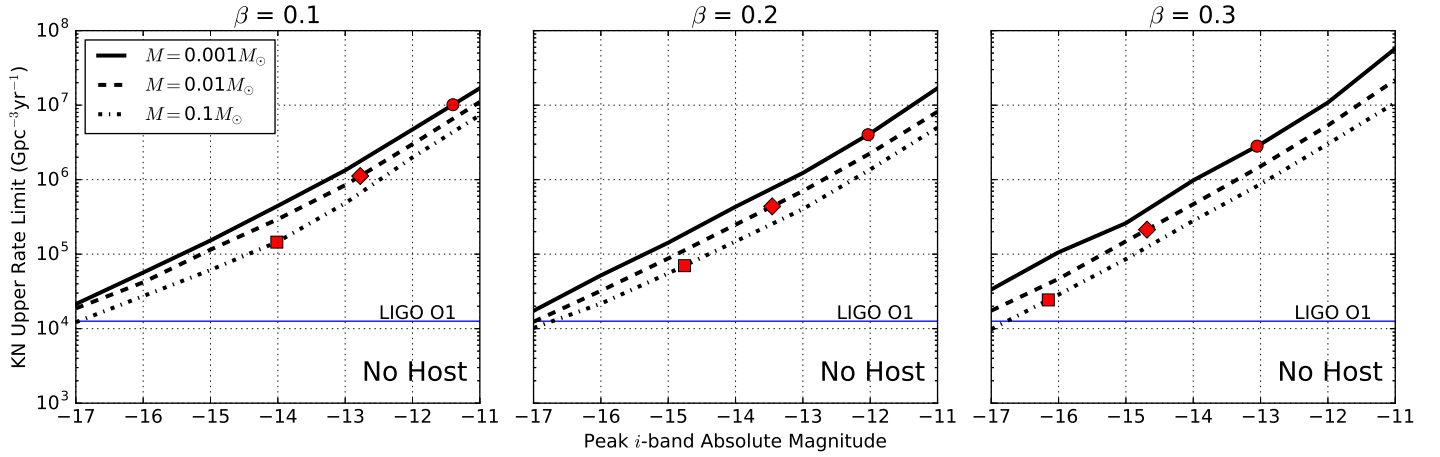
Figure 13. The 90% upper rate limit for the nine BK13 models using efficiencies calculated with SNANA . Each BK13 model is offset in absolute magnitude and the search efficiency is determined to calculate the rate. The red points show the rate limits for each model with no magnitude offset. The blue line shows the upper limit set in Advanced LIGO O1 (The LIGO Scientific Collaboration et al. 2016).
