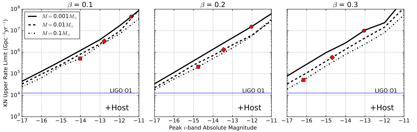
Figure 14. The same as Fig. 13, except using DiffImg efficiencies accounting for the SB anomaly.
