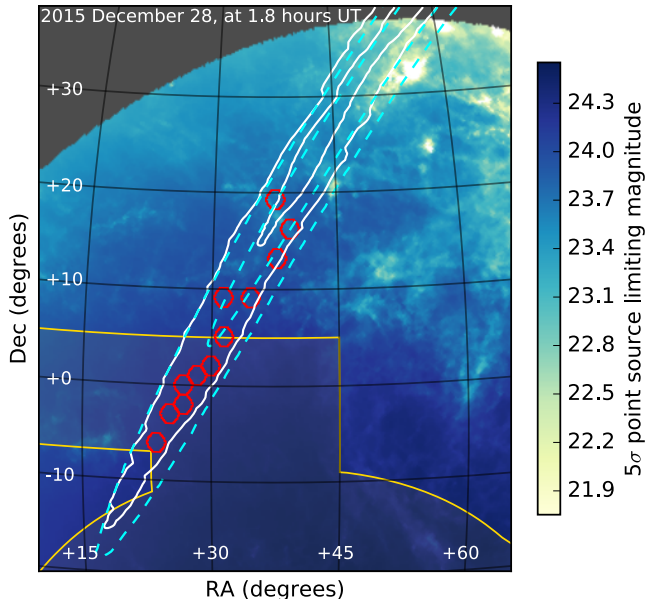
FIG. 1.— Sky region covered by our DECcam observations (red hexagons) relative to the 50% and 90% probability regions from the BAYESTAR (cyan contours) and LALInference (white contours) localization of GW151226. The background color indicates the estimated 5\sigma point-source limiting magnitude for a 90 s i -band exposure as a function of sky position for the first night of our DECcam observations. The variation in the limiting magnitude is largely driven by the dust extinction and airmass at that position. The dark grey regions indicate sky positions that were unobservable due to the telescope pointing limits. The yellow contour indicates the region of sky covered by the Dark Energy Survey (DES). The total effective area for the 12 DECcam pointings is 28.8 \text{ deg}^2 , corresponding to 3% (2%) of the probability in the BAYESTAR (LALInference) sky map.
