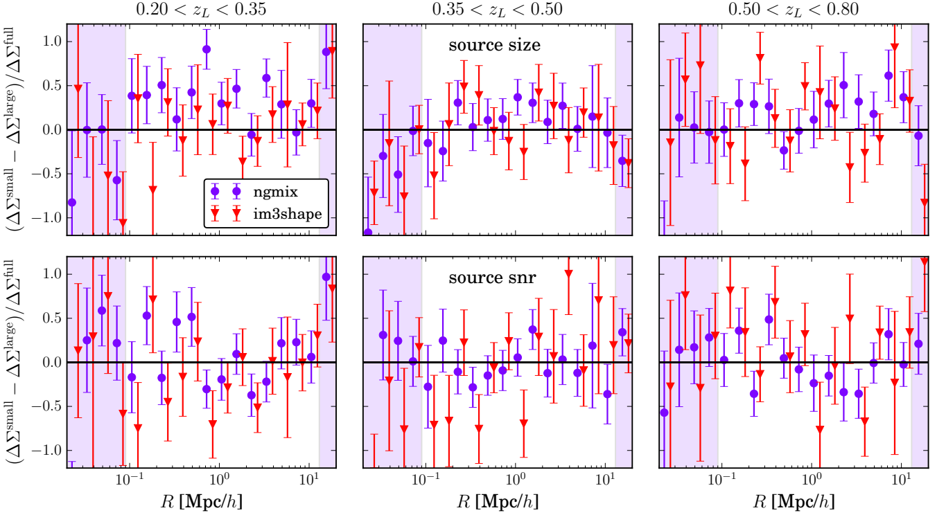
Figure 4. ( upper panels ): The difference between the shear of small and large source galaxies relative to the central values of the full sample for ngmix (purple circles) and im3shape (red triangles), measured for all three lens samples. ( lower panel ): The same, but showing results for the split between low and high signal-to-noise sources. These splits are not always consistent with zero, see the text in Sec. 5.3 for a detailed discussion.
