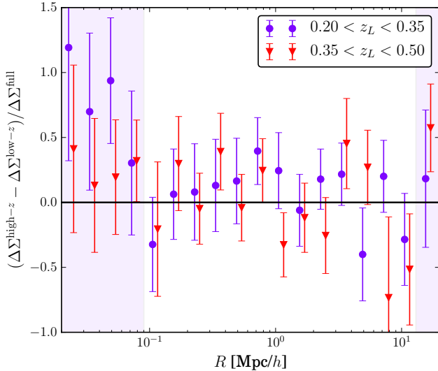
Figure 6. Same as Fig. 4 but showing the effect of splitting the ngmix sources into medium ( 0.55 < z_s < 0.83 ) and high redshift ( 0.83 < z_s < 1.30 ) bins. The result is shown for two lens redshift bins, 0.2 < z_L < 0.35 (purple circles) and 0.35 < z_L < 0.5 (red triangles). It is consistent with zero for both lens redshift bins.
