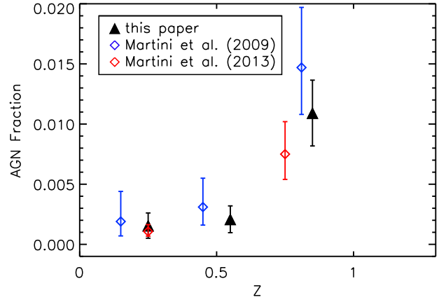
Figure 3. Comparison of the evolution of the AGN fraction in clusters with redshift in our sample and in previous work. For all samples only AGN with X-ray luminosity of L_X > 10^{43} \text{ erg s}^{-1} are included. The results of this paper are shown in black, for three separate redshift bins of 0.1 < z < 0.4 , 0.4 < z < 0.7 , 0.7 < z < 1.0 (black filled triangles). Also shown are the AGN fraction for Martini et al. (2009) for z -bins of 0.1 < z < 0.3 , 0.3 < z < 0.6 , 0.6 < z < 1.3 (blue diamonds) and the results of Martini et al. (2013) for z < 0.5 and 0.5 < z < 1.0 (red diamonds). Here we show the results for our sample for clusters with a richness threshold of \lambda > 20 as the samples of Martini et al. (2009, 2013) include primarily more massive systems.
