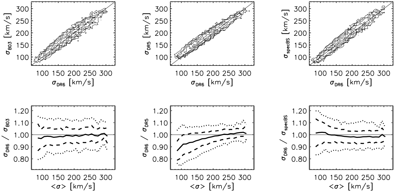
FIG. 7.— Top panels: velocity dispersion measurements from B03 (left), DR5 (middle) and specBS (right) versus the spectro1d DR6 values for the sample of elliptical galaxies used in Bernardi et al. (2003a). Bottom panels: The ratio of DR6 values to the other three samples (i.e. B03, DR5, and specBS ) versus the mean value (e.g. left panel \langle\sigma\rangle = (\sigma_{\text{DR6}} + \sigma_{\text{B03}})/2 ). The median value at each value of \langle\sigma\rangle is shown as a solid line; the values including 68% and 95% of the points are given as the dashed and dotted lines, respectively.
