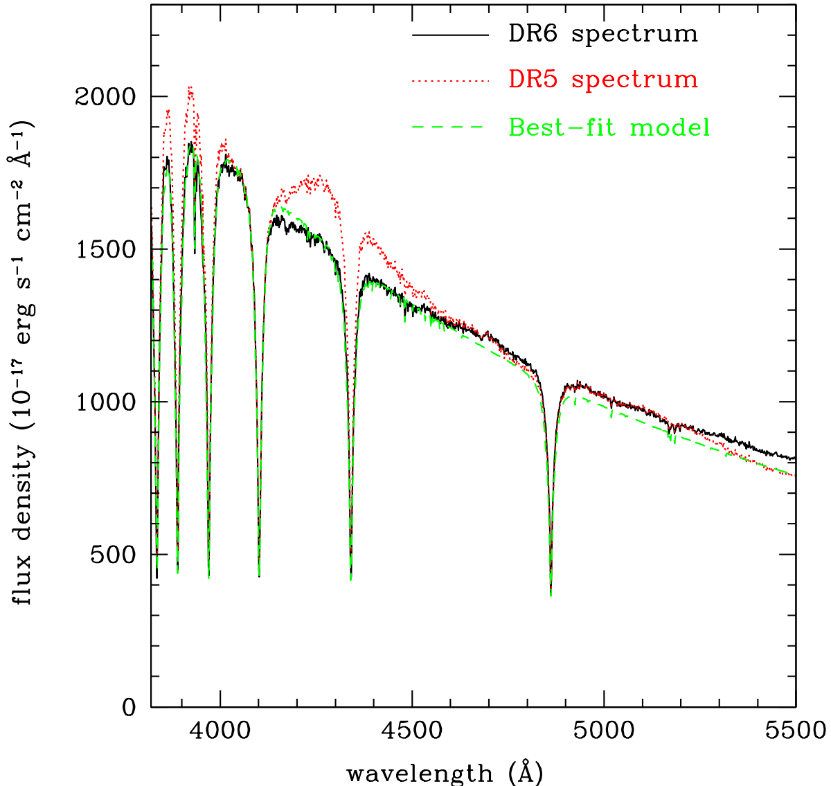
FIG. 6.— The blue part of the spectrum of an A0 blue horizontal branch star, SDSS J004037.41+240906.5, as given by the old (red dotted curve) and new (black solid curve) versions of idlSpec2d . The old curve has been scaled up by a factor of 1.24 (i.e., 0.35 mag), to reflect the difference in the calibration of the two reductions. The synthetic spectrum, shown in green, is generated from a model with parameters matching those derived from the SSPP ( T_{\text{eff}} = 8500 K, \log g = 3.25 , [\text{Fe}/\text{H}] = -2.00 ). The continuum between the absorption lines is much smoother, and matches the synthetic spectrum much better for the new reductions than for the old. The synthetic spectrum has been normalized to match the observed spectrum at 4500 Å. Neither the model nor the spectra have been corrected for Galactic reddening (which is E(B - V) = 0.036 in this line of sight).
