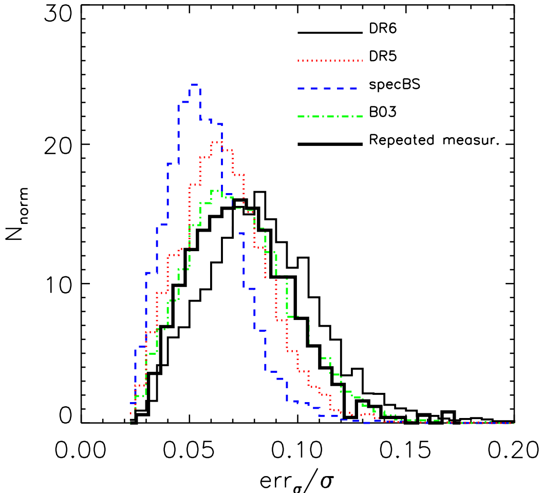
FIG. 8.— Error distribution of the velocity dispersion measurements from spectro1d DR6 (thin black solid line), spectro1d DR5 (dotted red line), specBS (dashed blue line), and B03 (dotted-dashed green line). The thick solid line was obtained by comparing the velocity dispersions of \sim 300 galaxies which had been observed two or more times; it is thus an empirical estimate of the true error.
