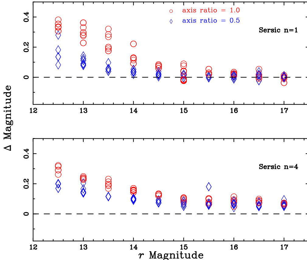
FIG. 6.— Difference between measured model and true r -band magnitudes of a series of simulated galaxies with Sérsic index of 1 (disk galaxies; upper panel) and 4 (elliptical galaxies; lower panel). These galaxies followed the magnitude-effective radius relation observed in the VAGC, and were either circularly symmetric (circles) or had an axis ratio of 0.5 (diamonds). They were added to random areas of real high-latitude fields, and run through photo . The simulated elliptical galaxies show a systematic offset even at the faint end; this is due to the fact that the photo model magnitude code assumes a truncation beyond 7 scale-lengths, while the “true” magnitude has no such truncation. This is a 0.05 mag effect.
