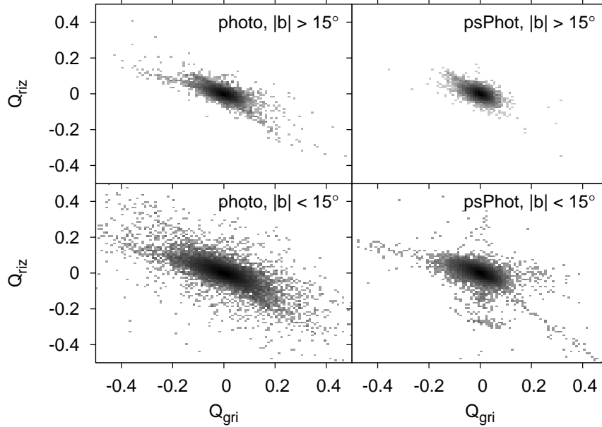
FIG. 4.— The distribution of median Q_{gri} and Q_{riz} parameters measuring the position of the stellar locus within each field for the photo (left) and PSPhot (right) photometric pipelines; zero values are indicative of uniform photometry. Within the Galactic plane (lower panels), the PSPhot values are more concentrated, but contain a higher number of systematic departures from the main locus. The PSPhot code in fact gives a tighter locus at high latitudes as well (upper panels). Histogram equalization of the gray-scale was used to emphasize low density regions.
