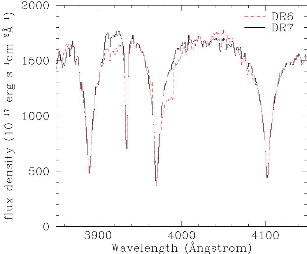
FIG. 9.— The spectrum of SDSS J172637.26+264127.6, an A0 star observed as part of SEGUE. The strong broad lines are due to Balmer absorption. The red dashed spectrum is that available in DR6, while the black solid spectrum is from DR7, with its improved flat-field.
