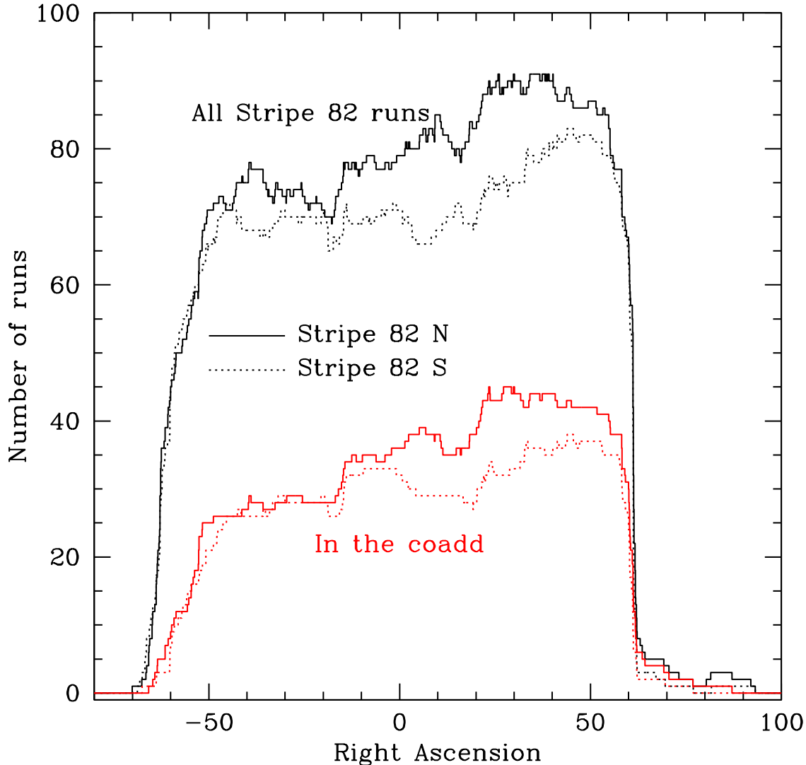
FIG. 3.— Stripe 82, the Equatorial stripe in the South Galactic Cap, has been imaged multiple times. The lower pair of curves show the number of scans covering a given right ascension in the North and South strip that are included in the coaddition (mostly data taken through 2005). In addition, Stripe 82 has been covered many more times as part of a comprehensive survey for 0.05 < z < 0.35 supernovae, although often in conditions of poor seeing, bright moon, and/or clouds; the total numbers of scans at each right ascension in the North and South strip are indicated in the upper pair of curves. All these data have been flux-calibrated, as discussed in the text, and are available (together with the coadd itself) in the stripe82 database.
