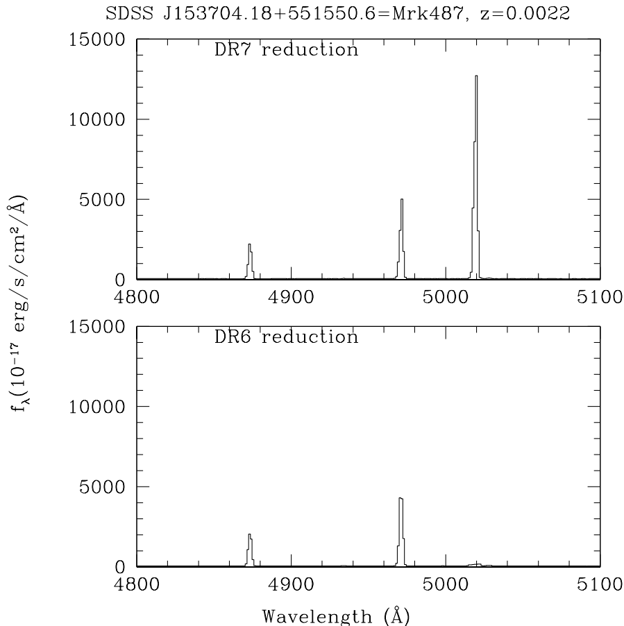
FIG. 10.— Spectra of the object SDSS J153704.18+551550.6=Mrk487, in DR6 and DR7. The stronger [OIII] emission line at 5020Å was mistaken for a cosmic ray and clipped away completely in DR6, while the weaker line at 4970Å was slightly affected. With the improved algorithm in DR7, the lines are not clipped.
