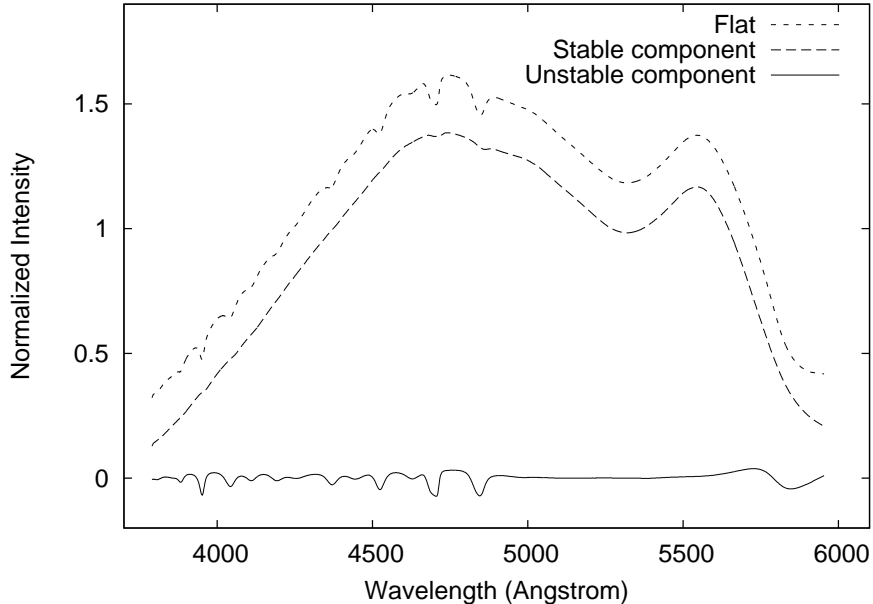
FIG. 7.— The decomposition of the flat field of the first blue spectrograph (upper curve) into stable (lower curve, offset slightly for clarity) and unstable (interference) components. The unstable component is close to zero, but shows wiggles at wavelengths that shift from one exposure to another.
