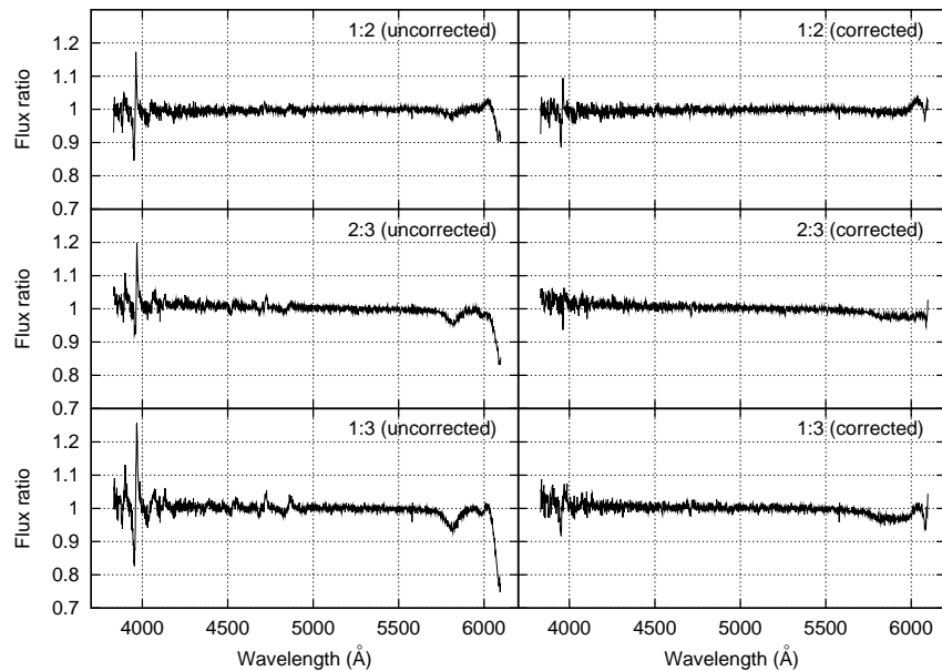
FIG. 8.— Median flux ratios over all objects in the three exposures of plate 1916, before (left) and after (right) correction for the moving interference filters. The ratio is fit to the derivative of the interference component of the flat field (Figure 7) after allowing for an arbitrary wavelength shift.
