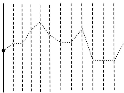
Figure 2: Many screens with many slits each. In the limit of infinitely many screens and infinitely many slits, the amplitude is the sum over all possible trajectories between the source and the observation point.
