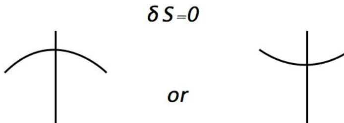
Figure 3: The pases add coherently on both sides close to the stationary action corresponding to the classical trajectory.
