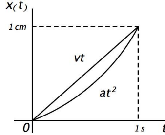
Figure 4: Classical trajectory for a free particle and an alternative non-classical one.
