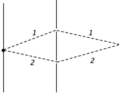
Figure 1: Double slit experiment. Different paths lead to different phases at the screen, which results in an interference pattern.
